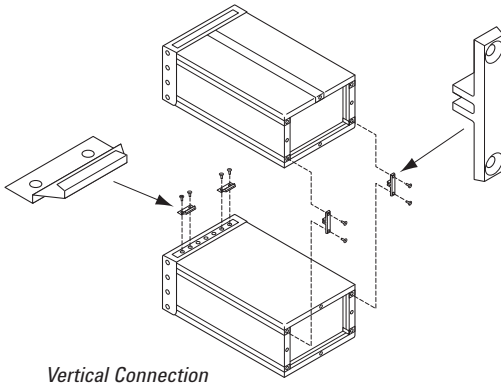
Vertical Connection
