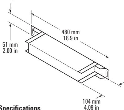
Ballast, alternate mounting (C2790AC)
