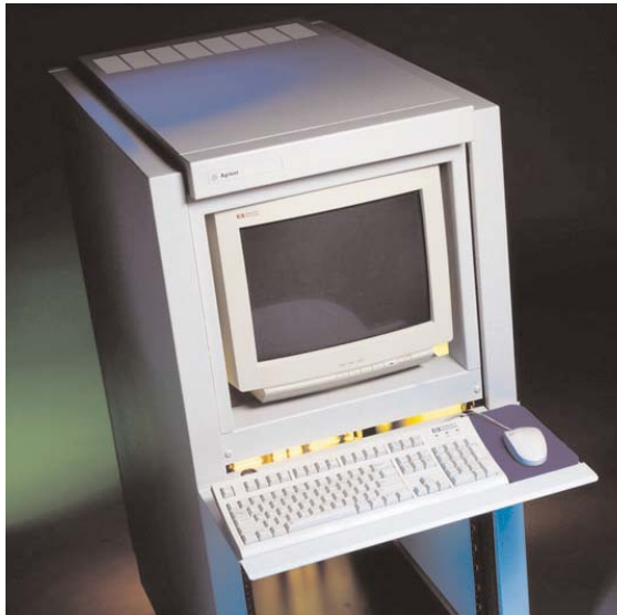
Monitor rackmount kit (J1519BC) installed with fixed keyboard kit (E7714AC) (monitor not included)
