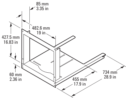
Monitor rackmount kit (J1519BC) installed with fixed keyboard kit (E7714AC) (monitor not included)
