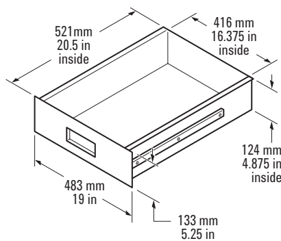
35181M Drawer
