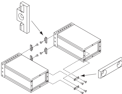
Side-by-side Connection
