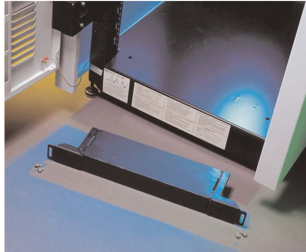
Ballast standard mounting (C2790AC)
